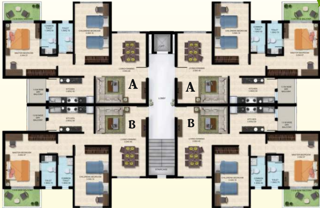
TYPICAL 2 BHK FLOOR PLAN
